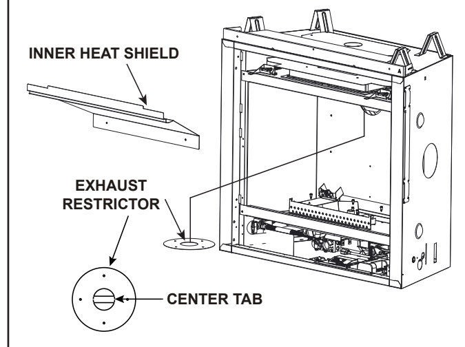
Figure 4.13 Exhaust Restrictor Installation
