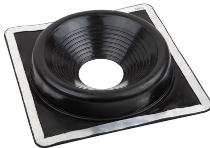
Corrugated and Metal roof Dektites
