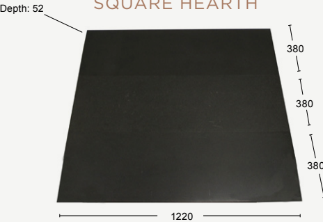
SQUARE HEARTH
